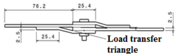
Fig -4: Line diagram Hybrid Lap joint with attachments
