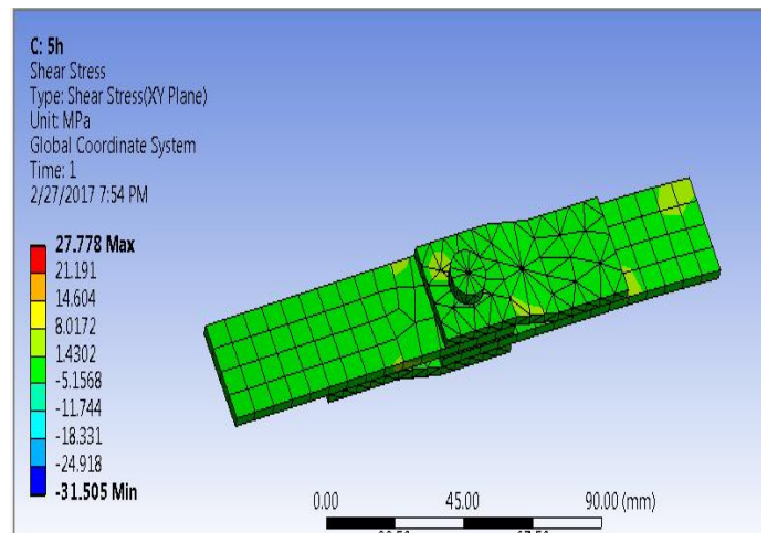
Fig -15: Shear stress of hybrid lap joint with load transfer distance of 5h curve attachment
