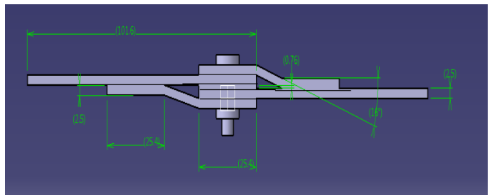
Fig -11: Geometric model of Hybrid lap joint with load transfer distance of 5h curve attachment.
