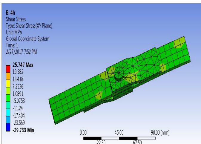
Fig -14: Shear stress of hybrid lap joint with load transfer distance of 4h curve attachment
