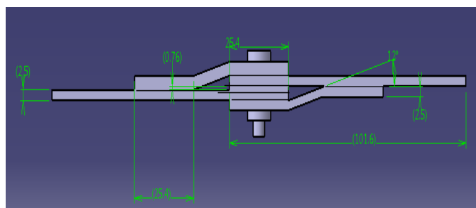
Fig -9: Geometric model of Hybrid lap joint with load transfer distance of 3h curve attachment.
