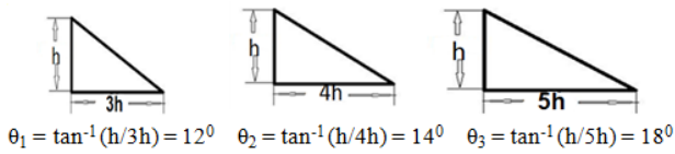
Fig -6: Variations in the load transfer triangle
