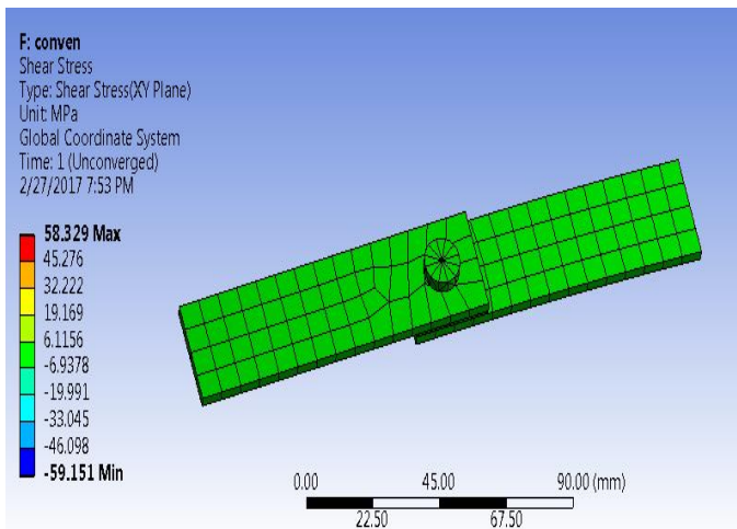
Fig -12: Shear stress of Conventional hybrid lap joint
