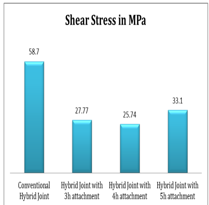
Chart -1: Shear stress of different joint configuration
