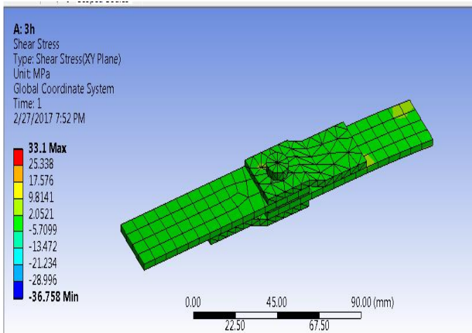
Fig -13: Shear stress of hybrid lap joint with load transfer distance of 3h curve attachment
