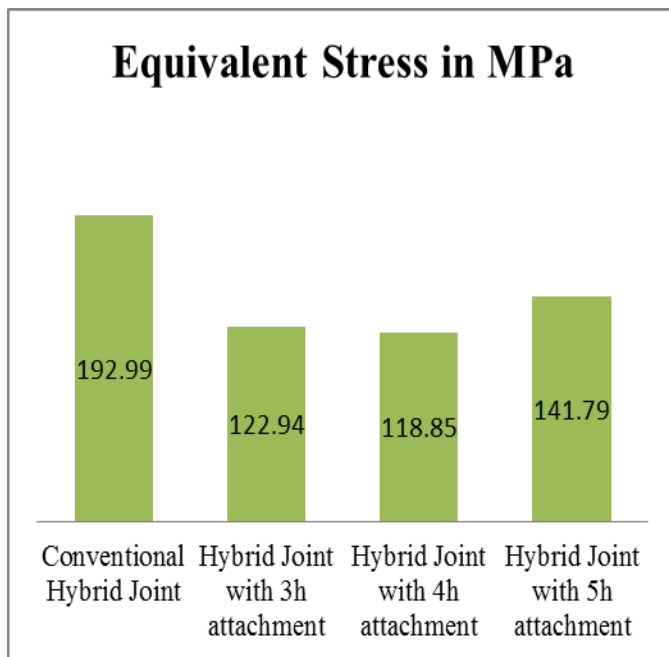
Chart -2: Equivalent stress of different joint configuration
