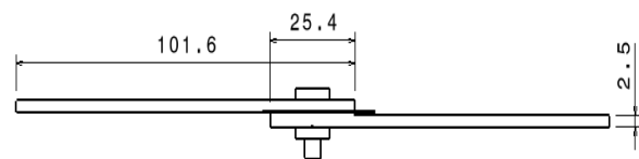
Fig -3: Line diagram of Conventional Hybrid Lap Joint
