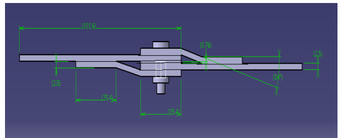
Fig -10: Geometric model of Hybrid lap joint with load transfer distance of 4h curve attachment.
