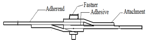
Fig -2: Hybrid Lap Joint with Curve Attachments
