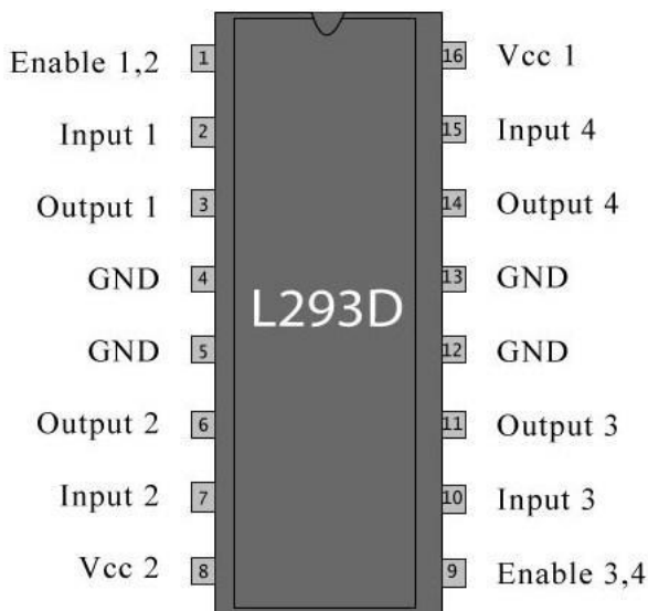
Fig -4: L293D pin Diagram
