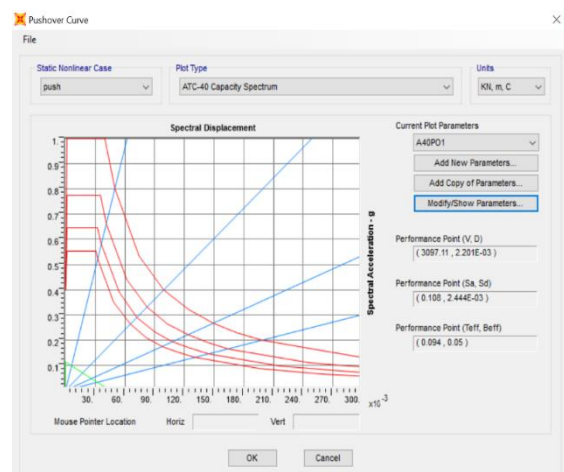
Fig-3 Capacity spectrum curve
