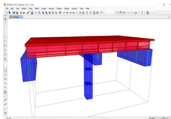
Fig-1: Model of the T-beam Bridge.
