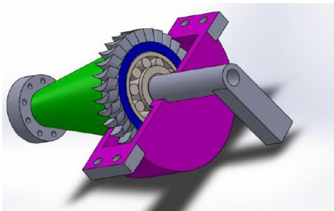
Fig -3: CAD model of Shaftless steam turbine
