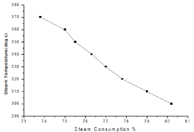
Fig -7: Effect of inlet steam temperature on steam consumption [11]
