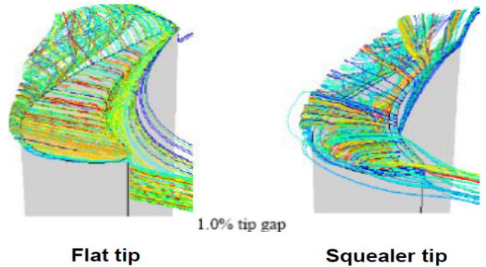
Fig -6: CFD analysis of blades
