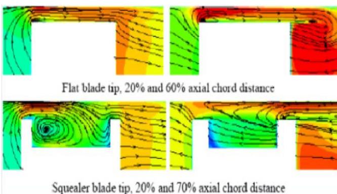
Fig -5: Analysis of Blade tip
