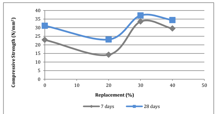
Graph - 1: Compressive Strength Values
