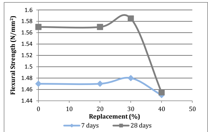
Graph -3: Flexural Strength Values
