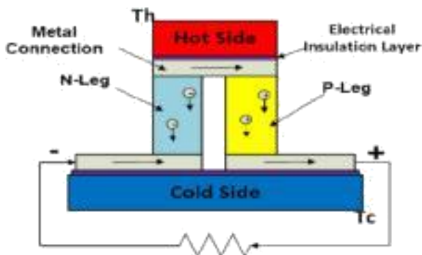
Fig.6. Simplified illustration of TEGs
