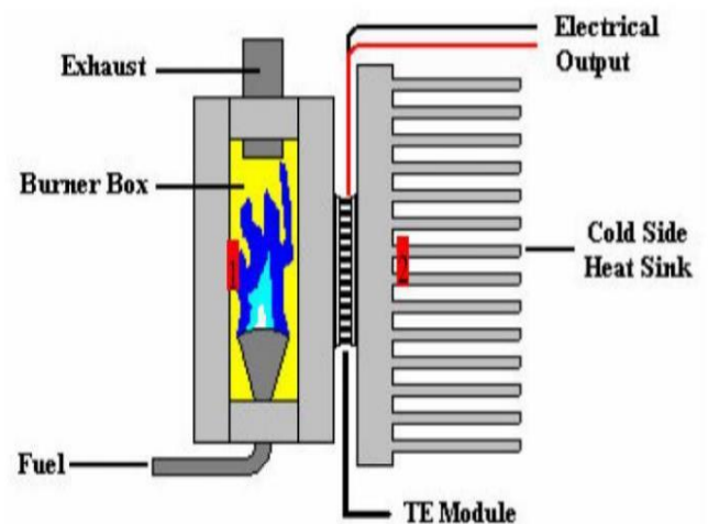
Fig.1 TEG utilizing the exhaust gas heat
