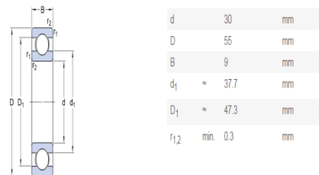
Fig.4: Bearing Specifications
