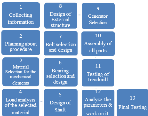
Fig. 2: Flowchart
