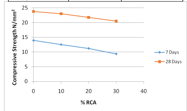
Fig. 4.1.1 Variation of Compressive strength with % RCA
