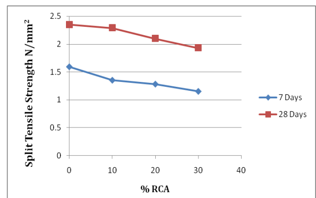
Fig. 4.2.1 Variation of split tensile strength with % RCA
