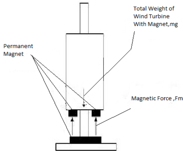
Figure 1: Free body diagram of magnetically levitated object
