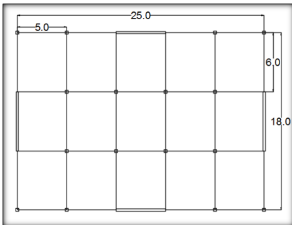
Fig-4 : Structural Layout.
