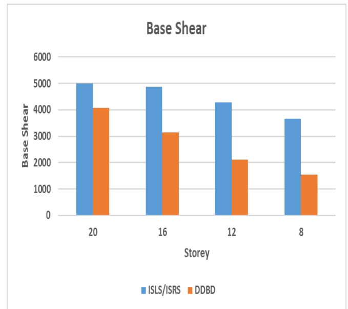
Chart-1 : Comparison of Base Shear Between DDBD & FBD
