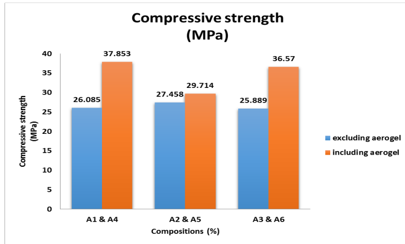
Fig. 7: Comparison of compressive strength with different compositions
