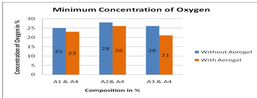
Fig. 6 : Comparison of with and without aerogel composite.
