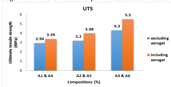
Fig. 8: Comparison of Ultimate Tensile Strength for different compositions
