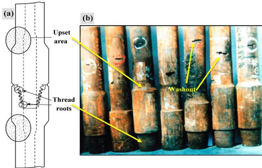
Fig. 1. (a) Critical regions of the drill pipe and connection causing fatigue failure [1], and (b) washout failure of the drill pipe transition zone
