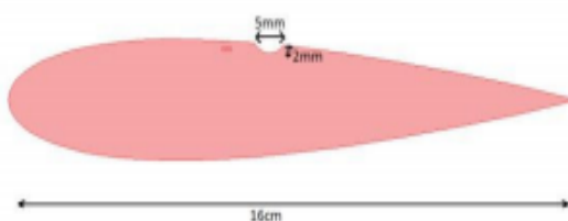
Fig. 1.2- NACA 008 Airfoil with Dimple
