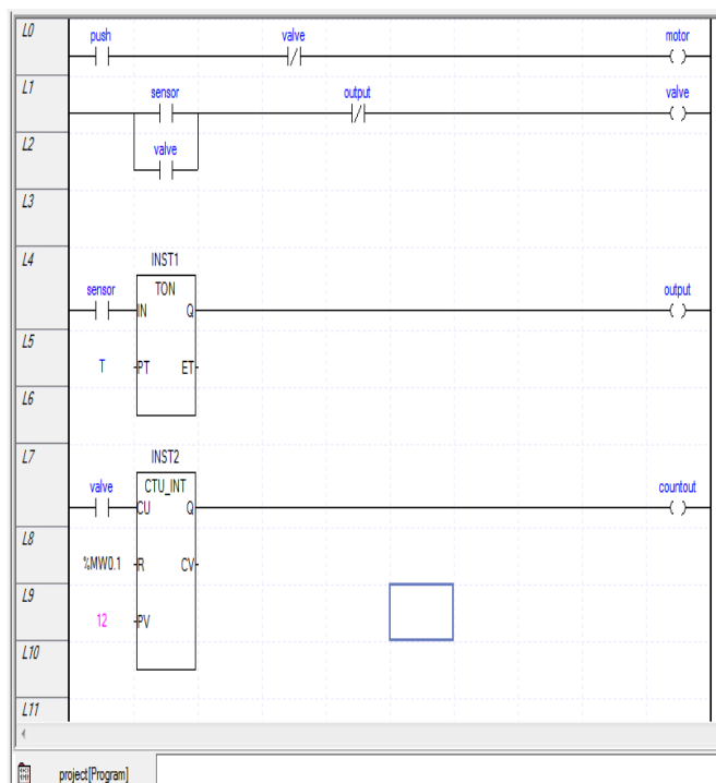
Fig-9: Overall software program using PLC
