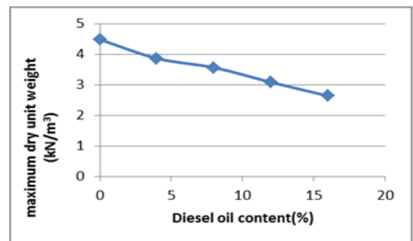
Chart - 3: Variation of Maximum Dry Density
