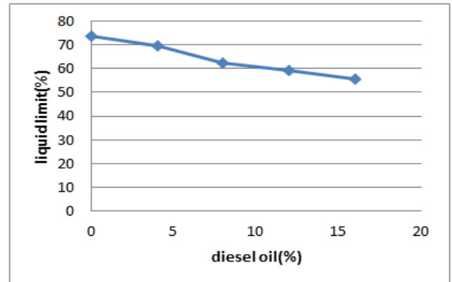
Chart -1: Variation of Liquid Limit
