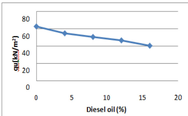
Chart -5: Variation of UCS with Diesel Oil
