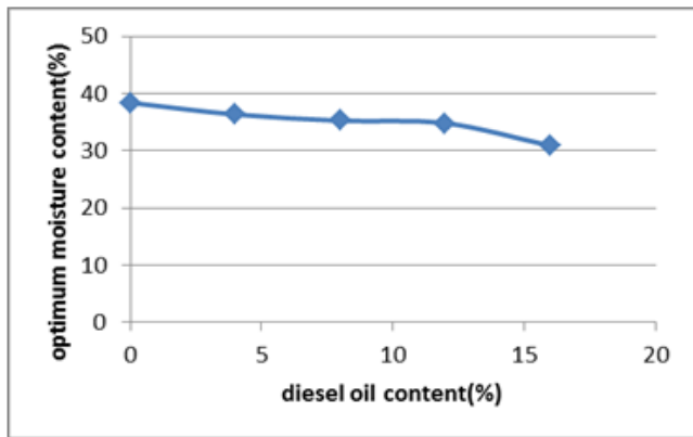
Chart - 4: Variation of Optimum Moisture Content
