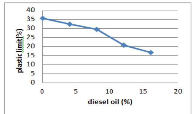
Chart -2: Variation of Plastic Limit
