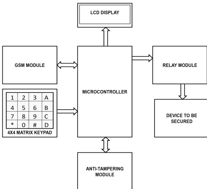
Fig. 2: Block Diagram of the Smart Security Lock
