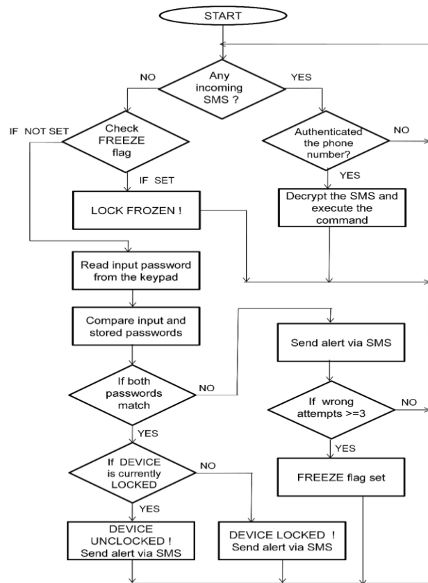
Fig. 3: Top Level Flowchart of the System
