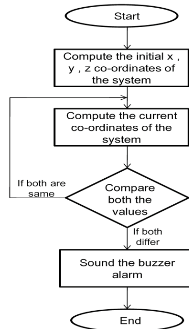
Fig. 4: Flowchart of the Anti-Tampering Module
