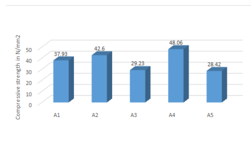
Fig.: Compressive Strength test results (ALKALINITY TEST)
