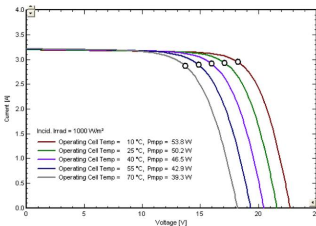
Fig -2: Output I-V characteristics of the PV module at various temperatures [1]
