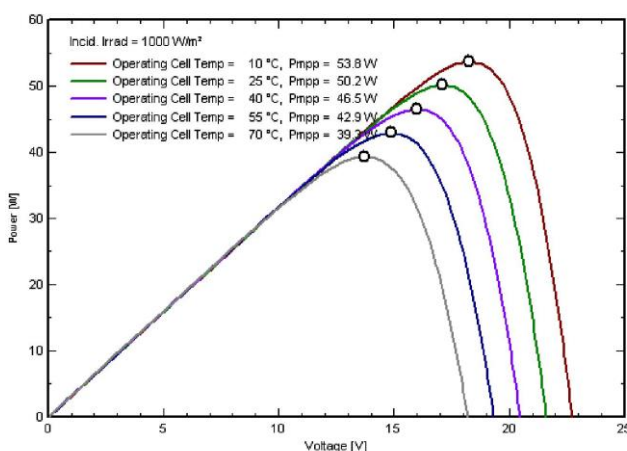
Fig -3: Output P-V characteristics of the PV module at various temperatures [1]
