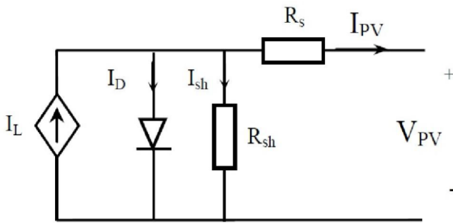
Fig -1: Equivalent circuit of PV-cell [1]
