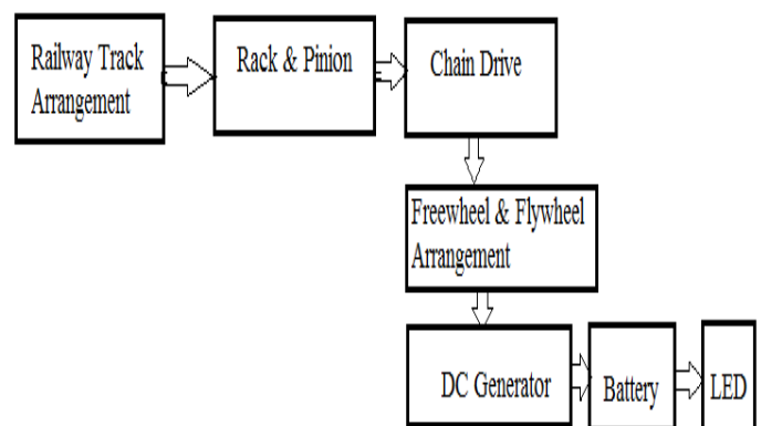
Fig.-1 Block Diagram of Generation of Power Using Railway Track
