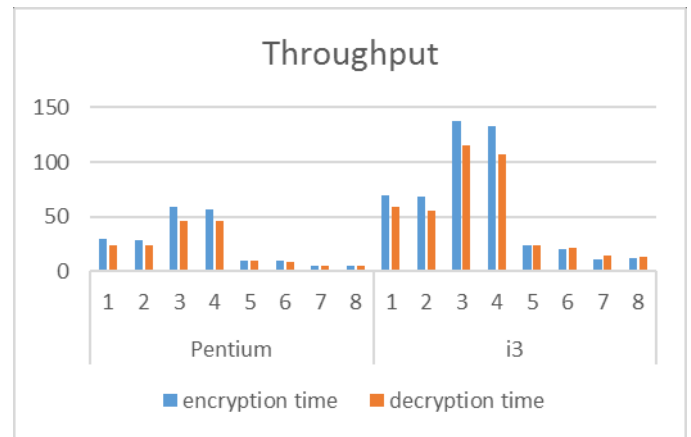
Fig -7: Graphical representation of throughput of AES algorithm for image file
