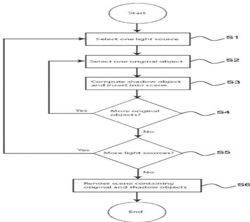
Flow Chart 4.1:Render Scene for original and shadow objects
