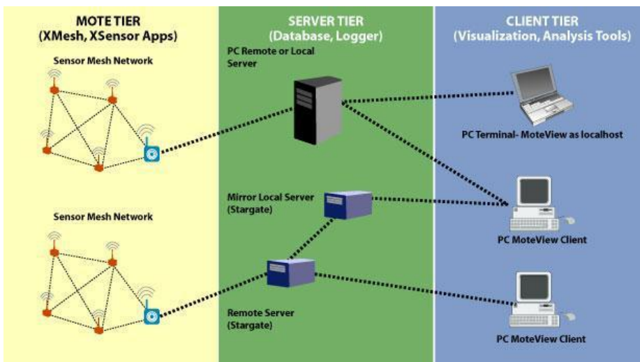
Fig 3.1:Mote View 3-Tier architecture
