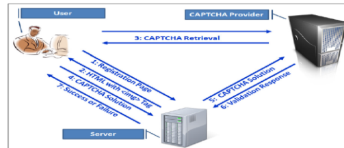
Fig- 2: A typical validation flow with CAPTCHA users
