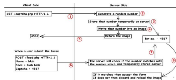
Fig-1: Working of CAPTCHA[5]
