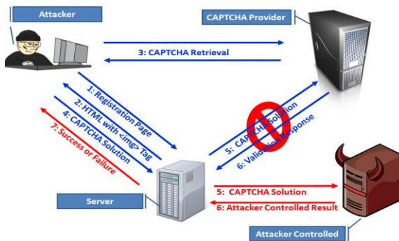
Fig-4: Image demonstrates CAPTCHA Clipping Attack
