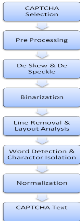
Fig-6: Steps involved in OCR Process for Text CAPTCHA
