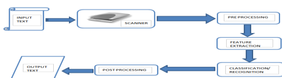
Fig-5: The basic Working of an Optical character recognition system.
