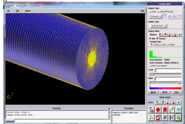
Fig 4. Nozzle Grid Generation With Circle Cross Section
