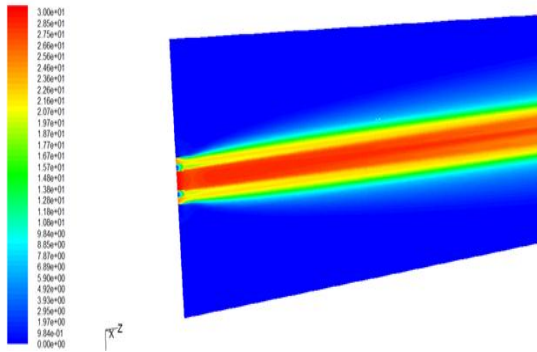
Fig 9. Circular Cross Section Without Annular
