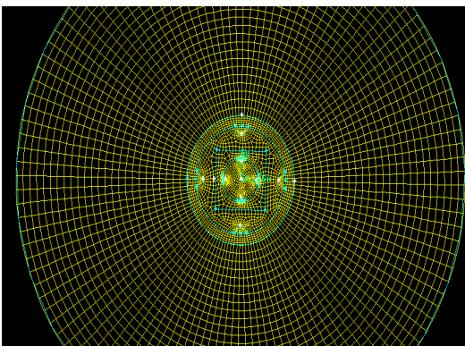
Fig 3. Nozzle Grid Generation With Square Cross Section
