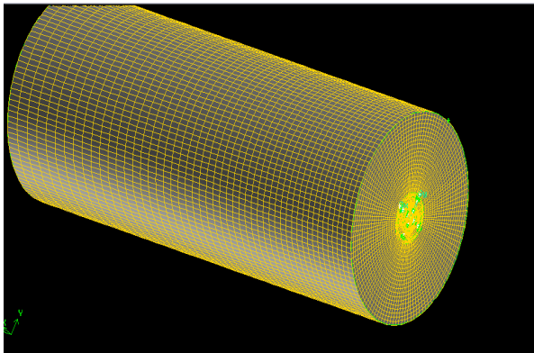
Fig 6 . Solid View Of Entire Domain With Element
