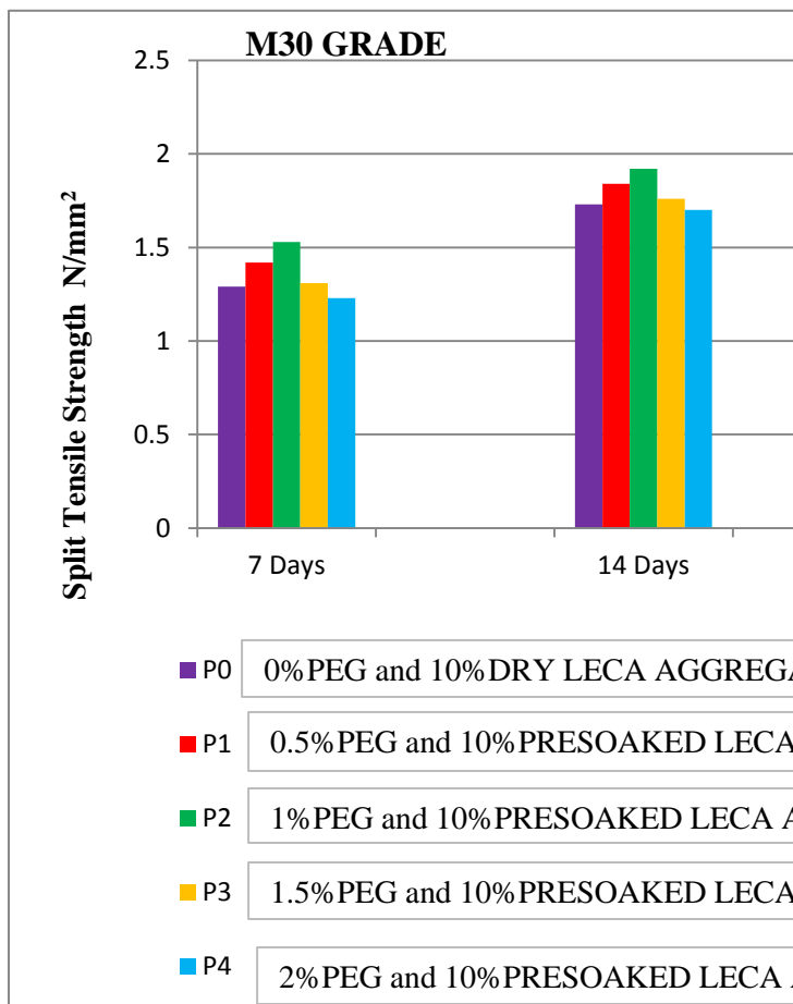
Graph 4- Split Tensile Strength For Different designation
