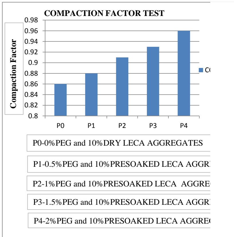
Graph-2 Compaction Factor Value for Different Designations
