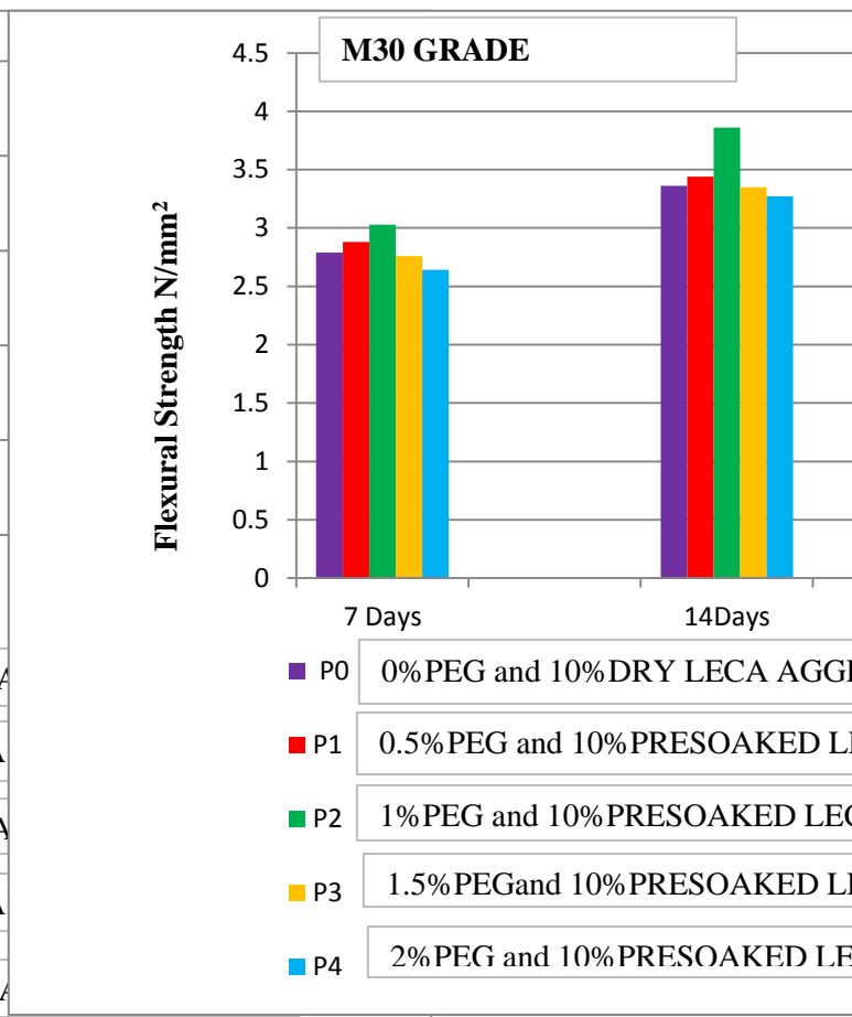
Graph 5-Flexural Strength for Different Designations.
