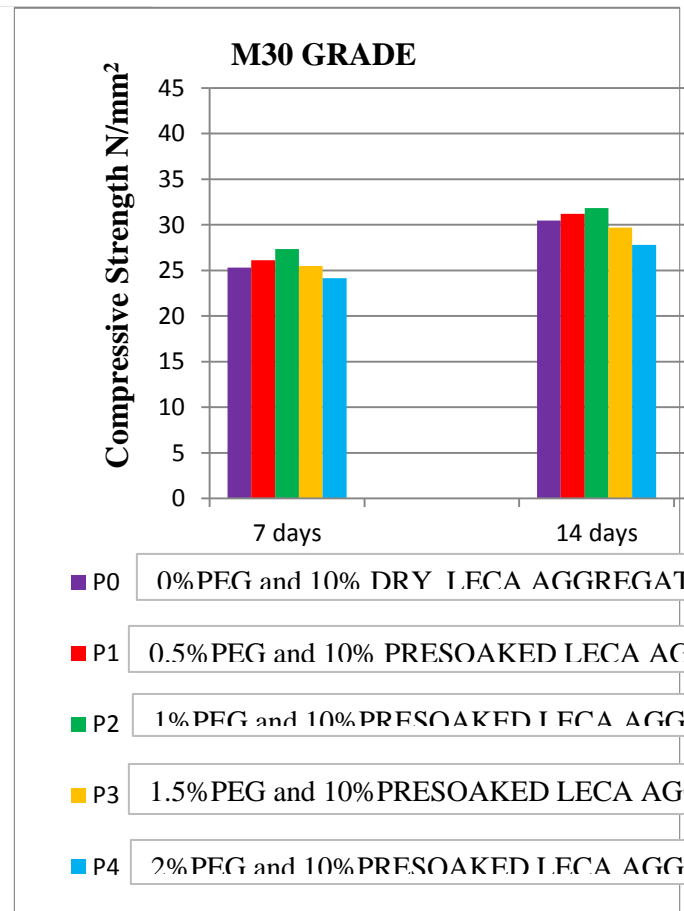
Graph 3- Compressive Strength for Different designation
