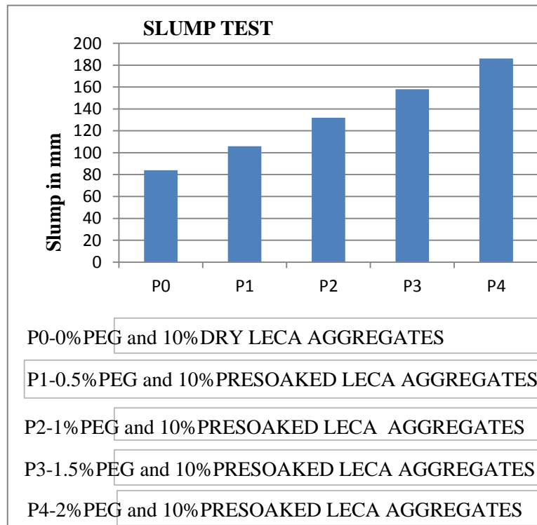
Graph-1 Slump Value for Different Designations
