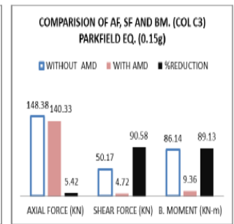
Fig. 5.12 Axial force, SF, BM for single AMD, for Parkfield Earthquake
