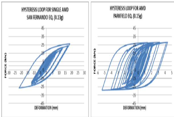
Fig 5.13 Hysteresis loop For San Fernando Earthquake Fig. Hysteresis loop for parkfield earthquake
