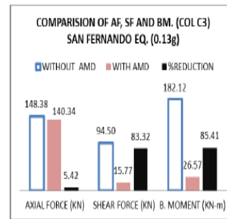
Fig. 5.11 Axial force, SF and BM for single AMD, for San Fernando Earthquake
