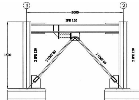
Fig.1.4b Application of AMD in seismic retrofitting of frames (based on Mehrtash MOTAMEDI, Fariborz NATEGHI-A., 2004)
