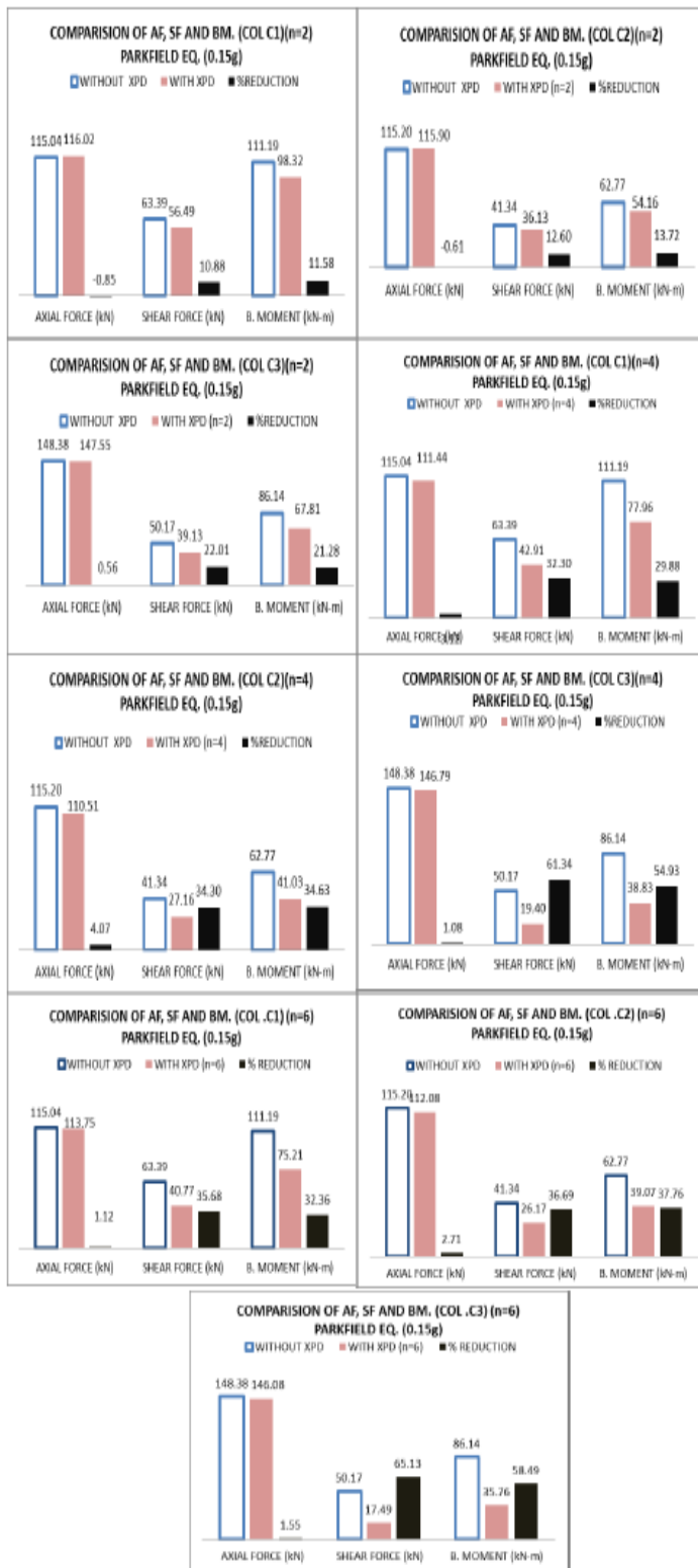
Fig. 5.5 Axial force, shear force and bending moment with XPD (n=2, 4 and 6) for column C1, C2 and C3 at top story of building for Parkfield Earthquake
