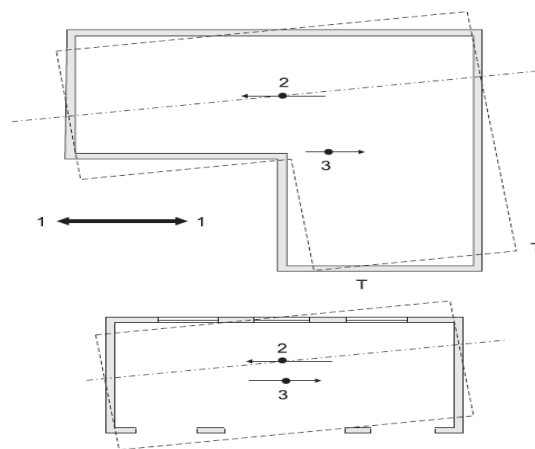
A. 1-Earthquake Force, 2-Centre of Stiffness Or resisting force ,3-centre of gravity ,T-Twisted building
