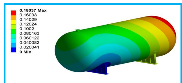
Figure-3 Maximum deformation- 0.18 mm
