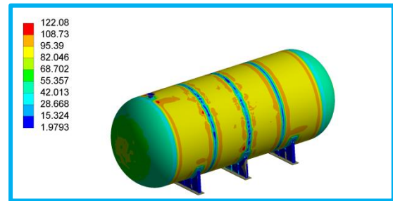
Figure-23: Stress=122.08 MPa
