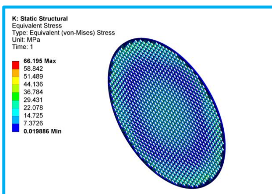
Figure-16 Maximum stress = 66.195 MPa
