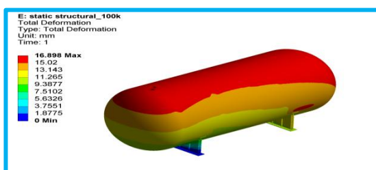
Figure-7 Maximum deformation= 16.89 mm
