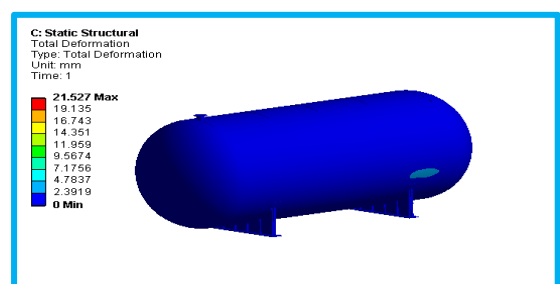
Figure-19: Deformation = 21.52 mm
