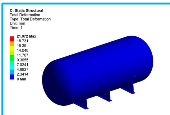
Figure-22: Deformation=21.072mm
