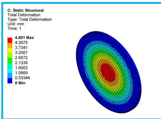
Figure-11 Maximum deformation= 4.801 mm
