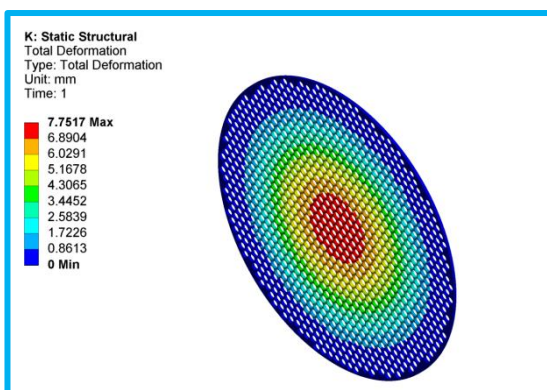
Figure-15 Deformation = 7.7517 mm
