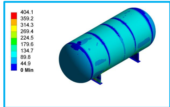
Figure-8 Maximum stress= 404.1 MPa
