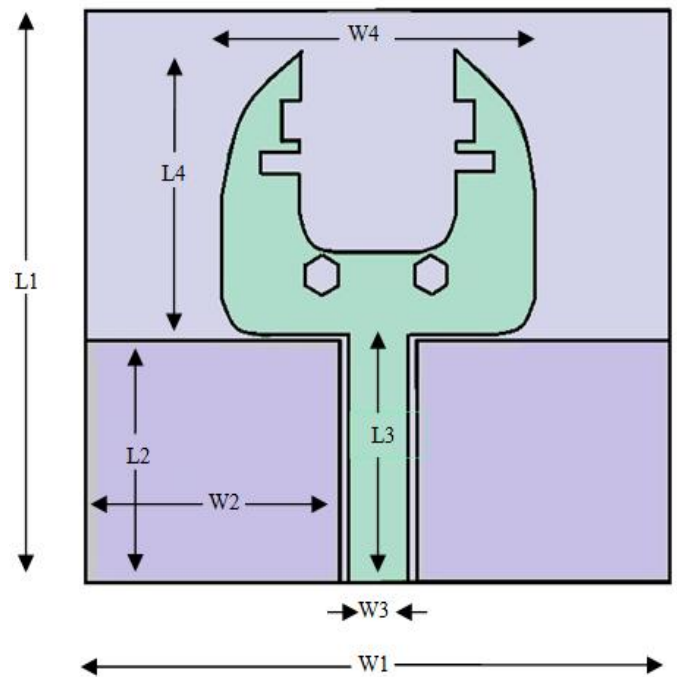
Fig-2: Geometry of the proposed antenna
