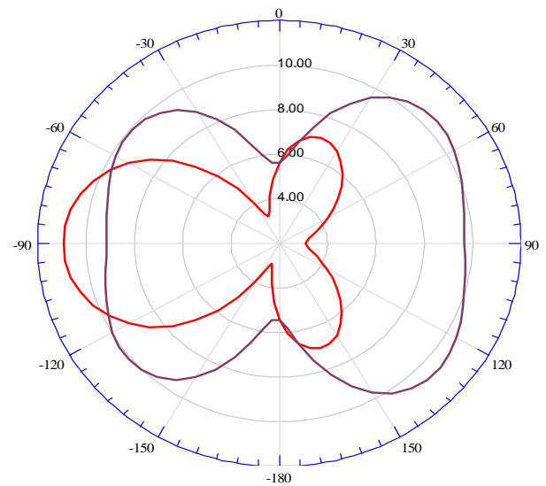
Fig -6: Radiation Pattern of proposed antenna at 9GHz
