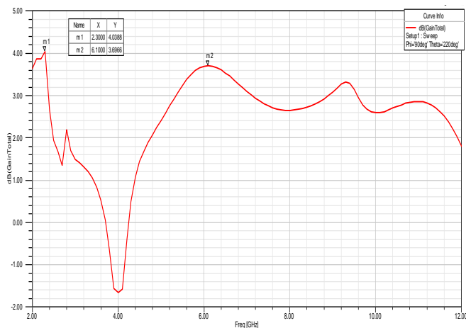
Fig-5: Total gain of proposed antenna
