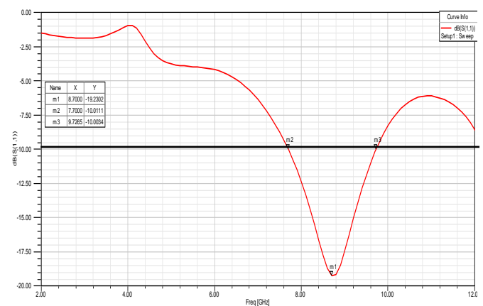
Fig-3: Simulated S11 characteristics of proposed antenna
