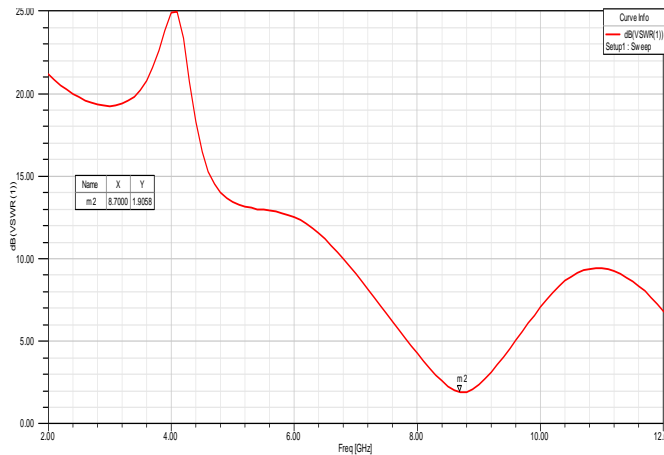
Fig -4: Simulated VSWR for the proposed antenna
