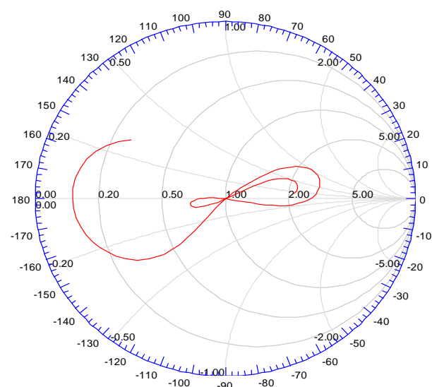
Fig-7: Smith chart plot of proposed antenna
