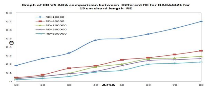
Fig -14: Graph Of CD Vs AOA For Comparison Of Re For Naca4421 -15 Cm Chord Length
