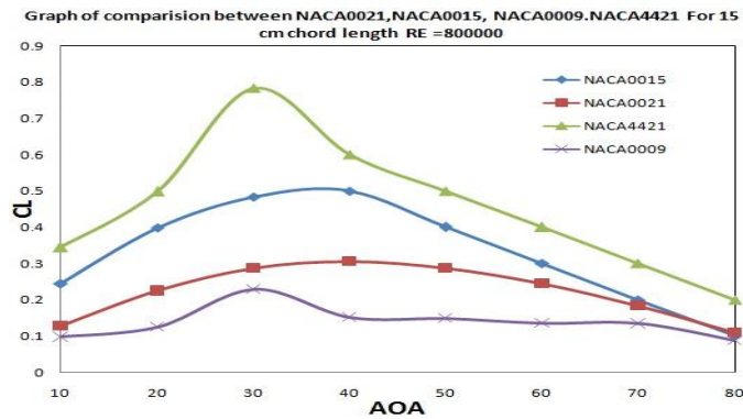
Fig -19: Graph Of CL Vs AOA For Comparison Of NACA0021 & NACA0015 for 15 cm Chord length and RE=800000
