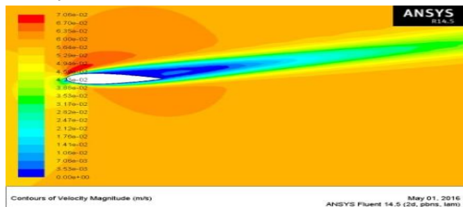
Fig -5: velocity counter for angle of attack 10^\circ
