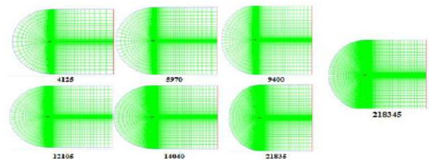
Fig -3: Grid independence study mesh
