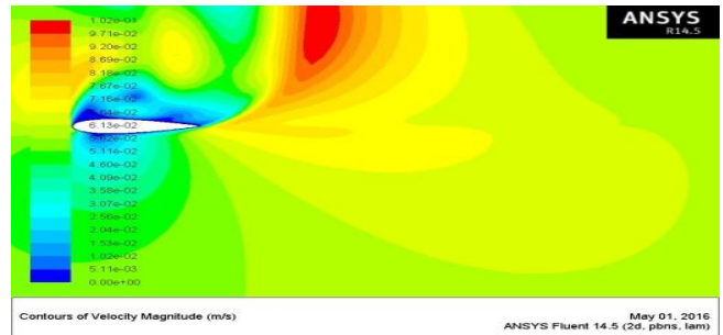
Fig -6: velocity counter for angle of attack 70^\circ
