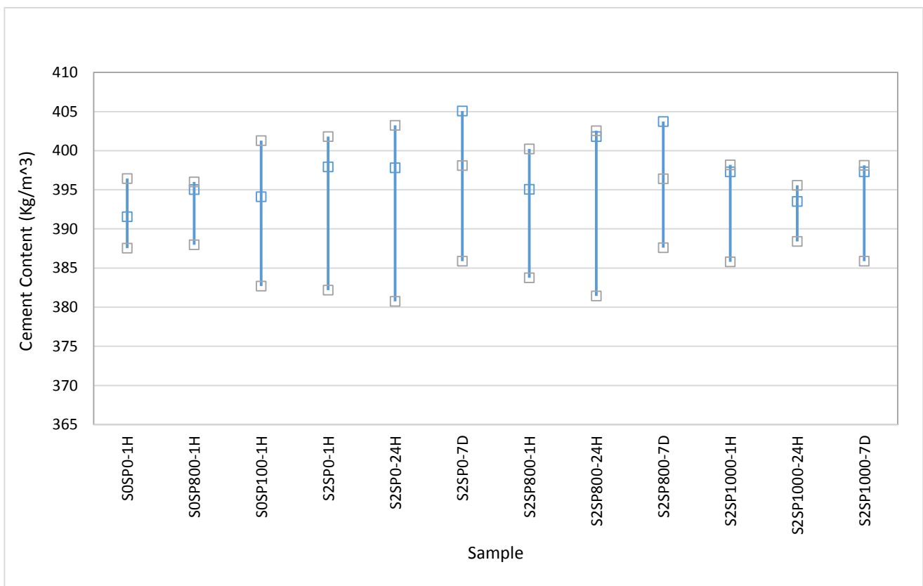
Chart -2 Variation of cement content for different delay times and different superplasticizer contents
