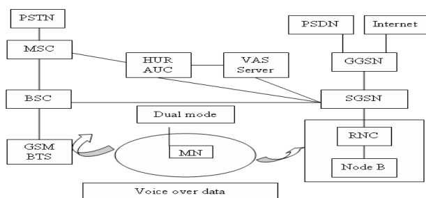
Figure 1.3 UMTS Architecture
