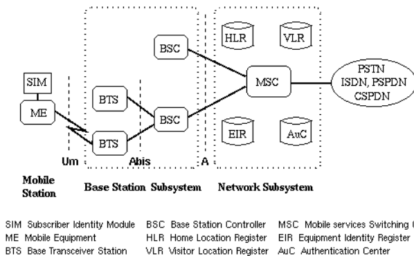
Fig1.2: CDMA Architecture
