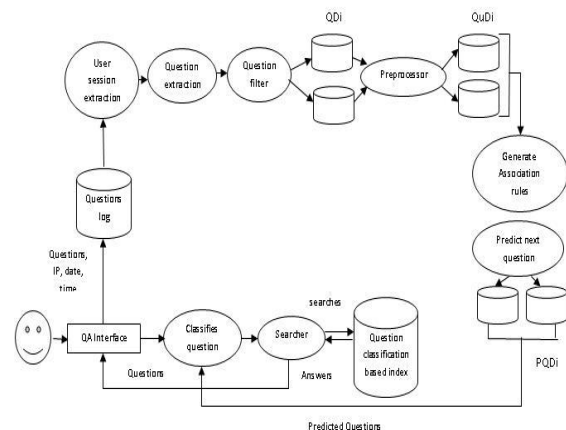
Fig. 4 Working of the system
