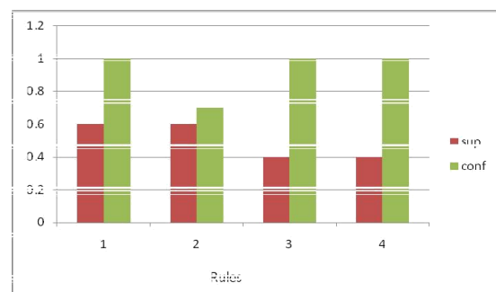
Fig. 3 Support and Confidence values
