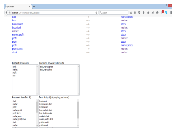
Fig. 7 The association rules generated after posting query
