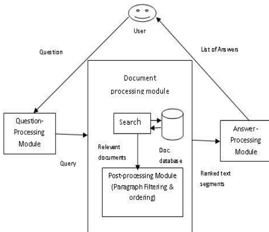
Fig.1 Architecture of Question answering system
