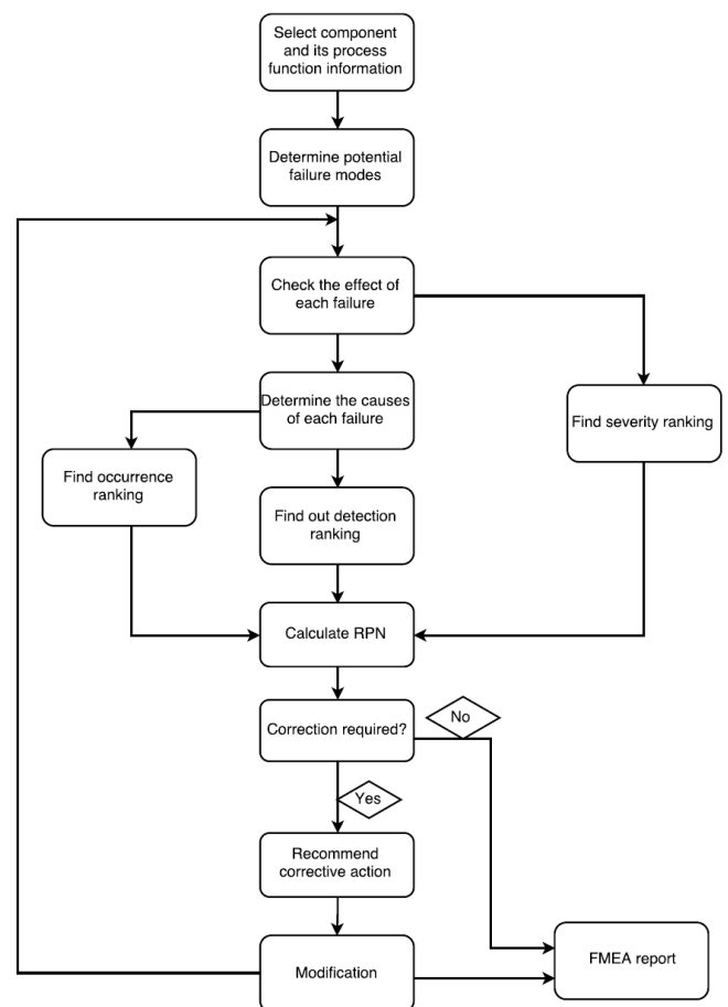
FLOW DIG. FOR FMEA PROCEDURE [13]
