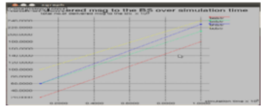
Figure 5.5 This plot shows the number of delivered message to the base station by forming cluster node.
