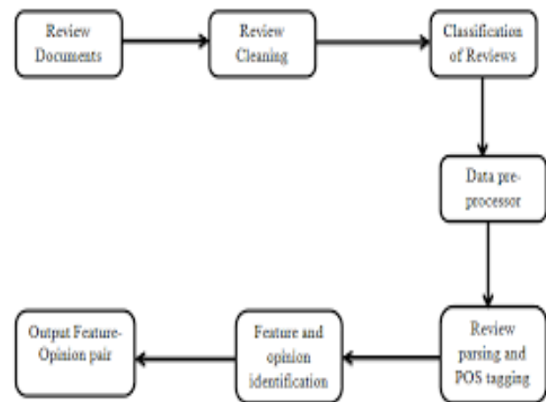
FIG-1.OPINION MINING SYSTEM
