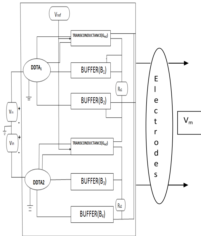
Fig-1: Architecture of Current Driver
