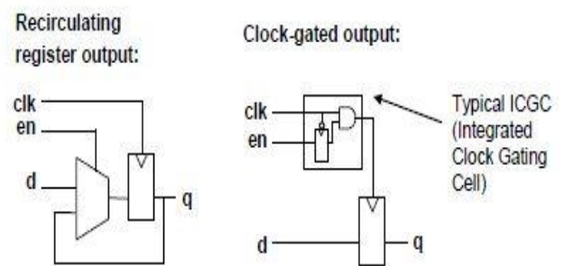
Fig 4.(a). Feedback mux Fig 4.(b). Integrated clock gating
