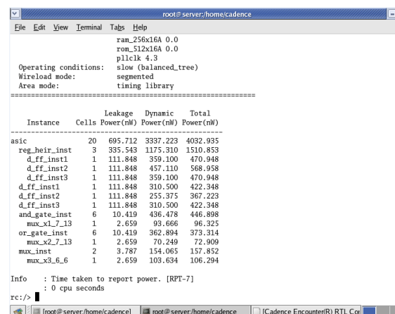
Fig 6(d). Before Asic Design RTL Power in Cadence Tool
