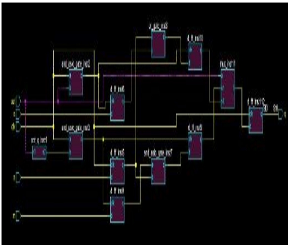
Fig 7(a). Clock gating Asic Design Schematic in Questasim Tool
