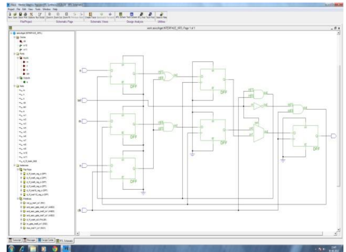
Fig 7(c). Clock gating Asic Design Schematic in Precision Tool
