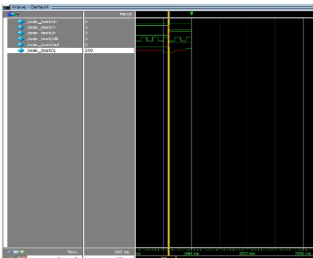
Fig 7(b). Clock gating Asic Design Wave Form in Questasim Tool
