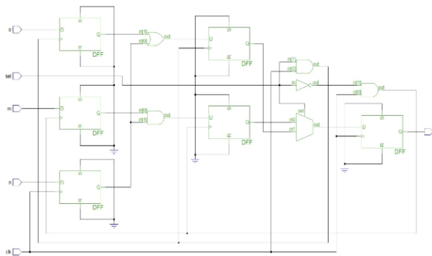
Fig 4. Clock gating in Asic Design
