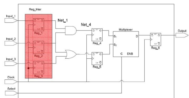
Fig1(a). Before guarded evaluation
