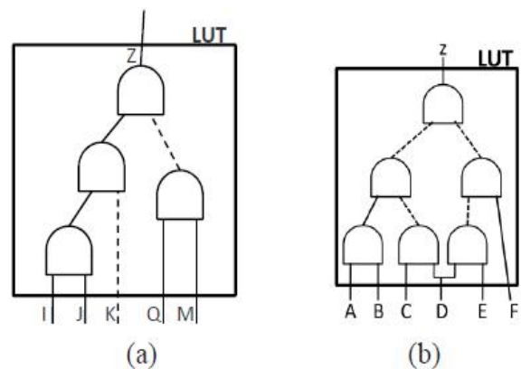
Fig 2.(a). Identifying gating inputs on LUTs using noninverting paths; Fig 2.(b). Identifying trimming inputs on LUTs using Partial non-inverting paths
