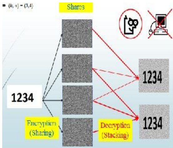
Fig. 1-Example of (k,n) cryptographic scheme
