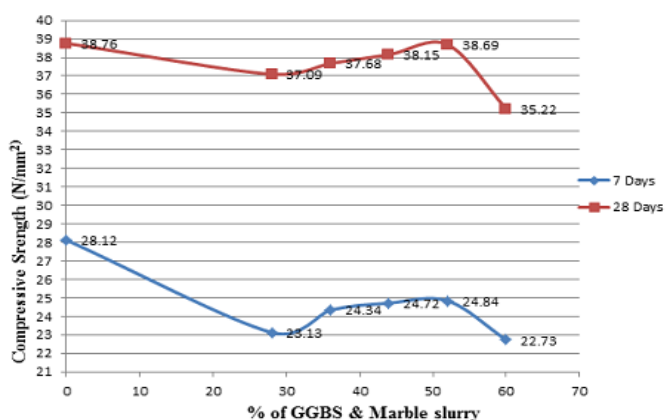
Chart-2 Effect of Ground-granulated blast-furnace slag and Marble slurry on Concrete of M25 Grade on Replacement for 7& 28 Days Compressive Strength of Cube
