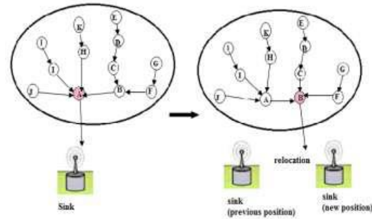
Figure 2: Relocating position of sink in WSN
