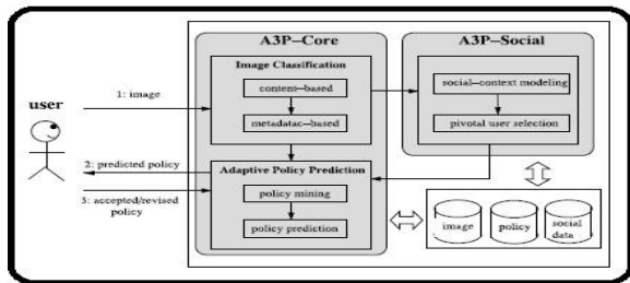
Fig.1. Framework of A3P
