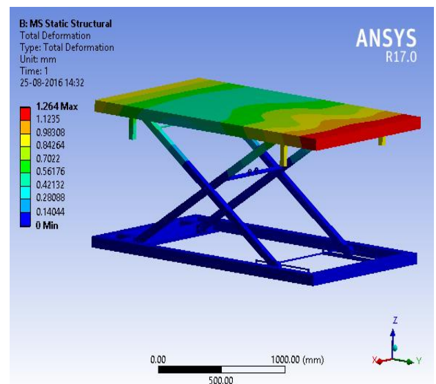
Fig.(13) Total Deformation of MS Hydraulic Scissor Lift, mm
