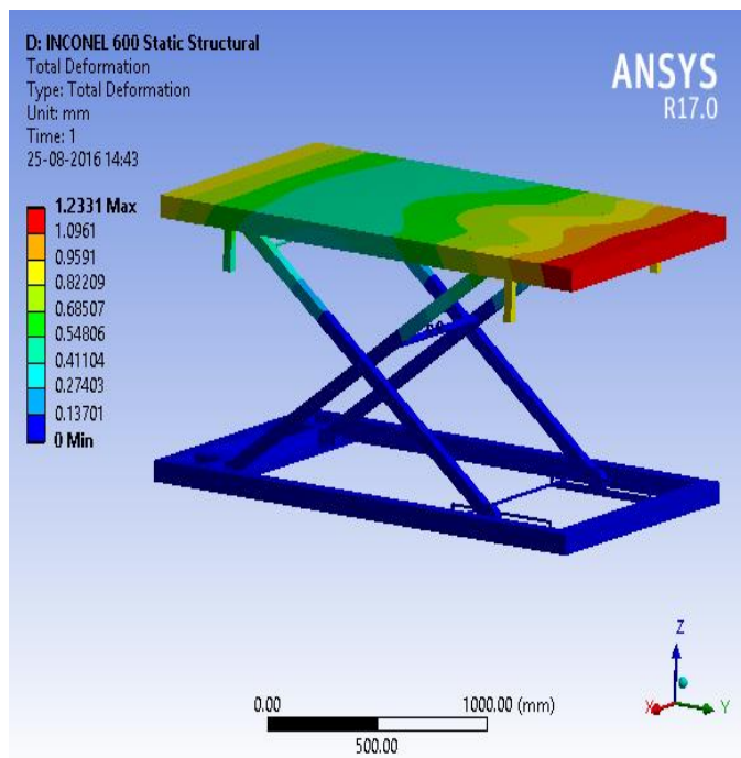
Fig.(21).Total Deformation of INCONEL 600 Hydraulic Scissor Lift, mm.
