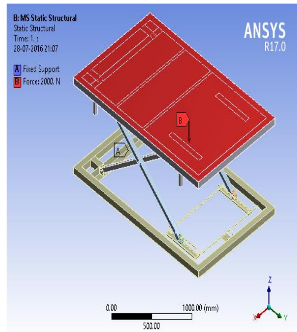
Fig.(10) FEA Model of Hydraulic Scissor Lift With Boundary Condition
