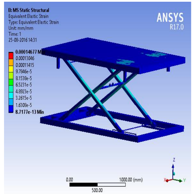
Fig.(12).Equivalent Elastic Strain of MS Hydraulic Scissor Lift.
