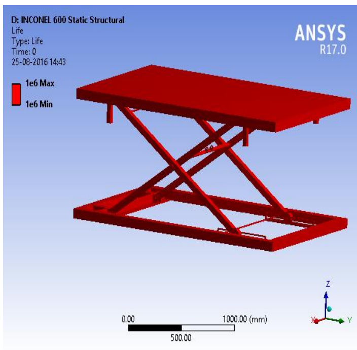
Fig.(22).Life of INCONEL 600 Hydraulic Scissor Lift.
