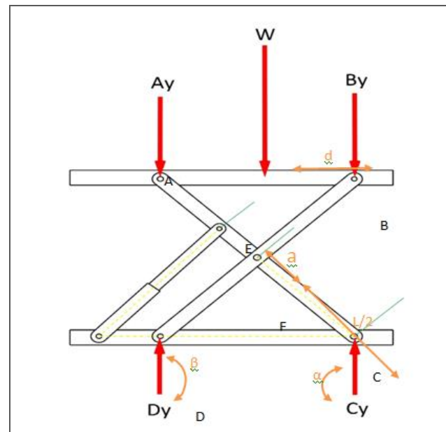
Fig.(6) Dimensions and Reactions of Forces
