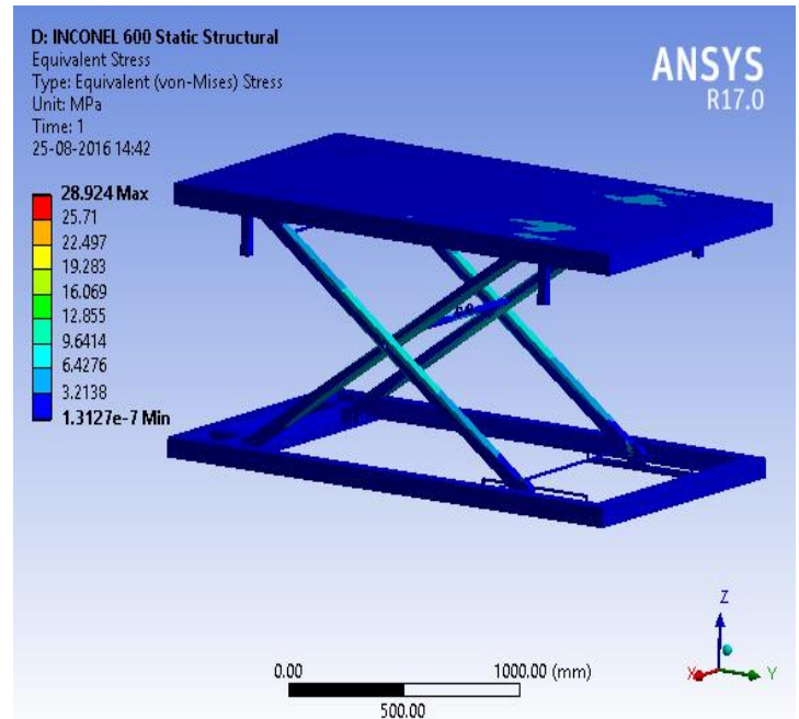
Fig.(19) Equivalent (Von-Mises) Stress of INCONEL 600 Hydraulic Scissor Lift,Mpa.
