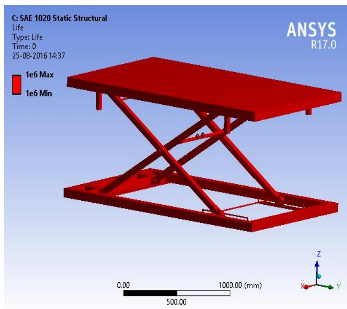
Fig.(18) Life of SAE 1020 Hydraulic Scissor lift
