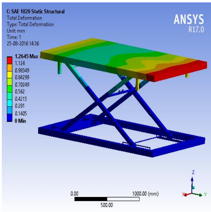
Fig.(17) Total Deformation of SAE 1020 Hydraulic Scissor Lift,mm
