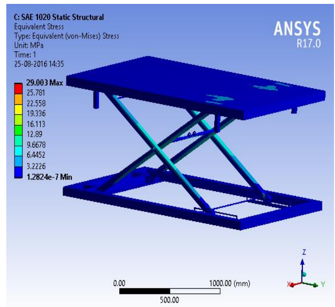
Fig.(15) Equivalent (Von-Mises) Stress of SAE 1020 Hydraulic Scissor Lift, Mpa
