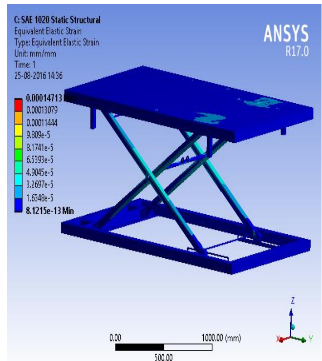
Fig.(16) Equivalent Elastic Strain of SAE 1020 Hydraulic Scissor Lift.
