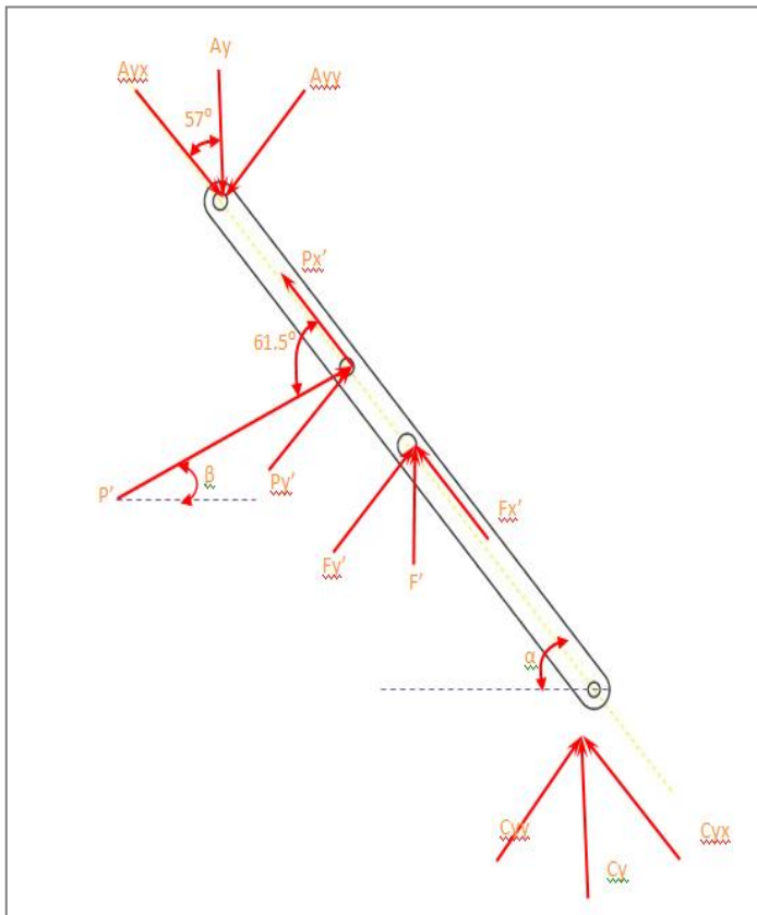
Fig. (7) Free Body Diagram of Arm
