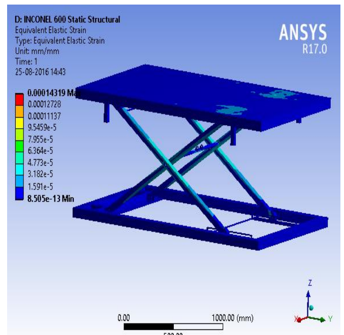
Fig.(20).Equivalent Elastic Strain of INCONEL 600 Hydraulic Scissor Lift.
