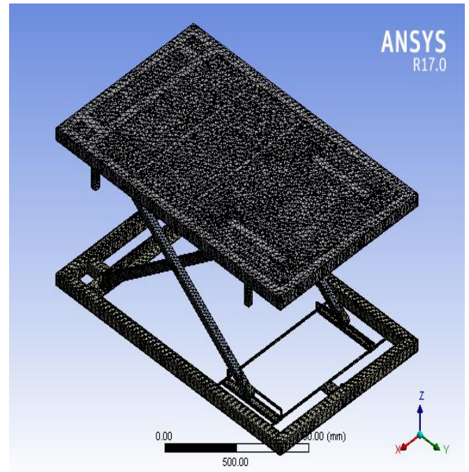
Fig.(9) FEA Model of Hydraulic Scissor Lift With Meshing.
