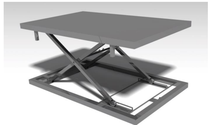
Fig. (1): Hydraulic Scissor Lift
