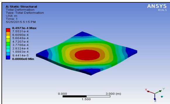
Fig.No.4: Deformation of Solid Flat Slab
