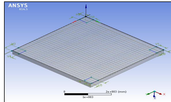
Fig.No.1: Solid Flat Slab Model
