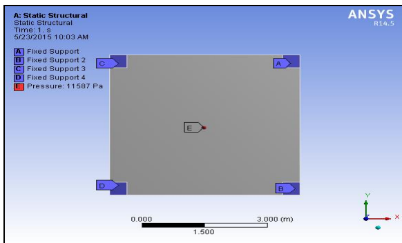
Fig.No.6: Loading Arrangement of Voided Slab
