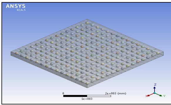
Fig.No.5: Voided Slab Model
