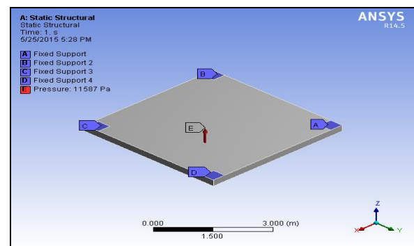
Fig.No.3: Loading Arrangement of Solid Flat Slab
