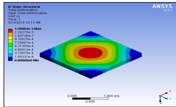
Fig.No.7: Deformation of Voided Slab
