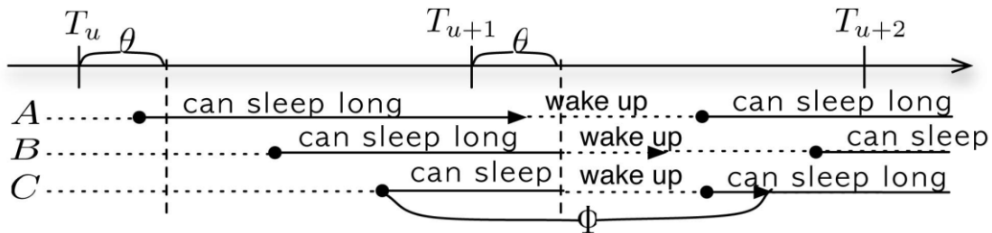
Fig. 4. Sleep mode in X-TESLA.
