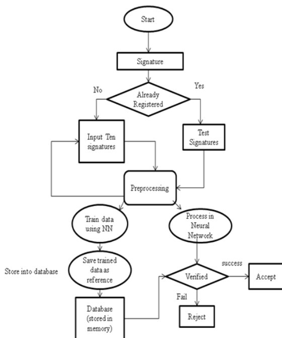
Fig -3: Signature Recognition & Verification
