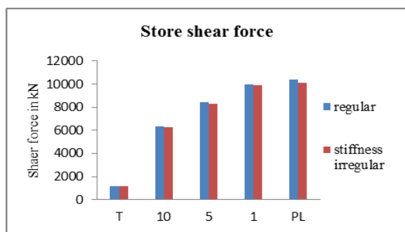
Chart -11: Storey shear force in X direction
