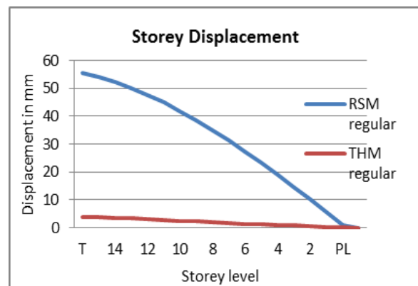
Chart -13: Displacement in X direction
