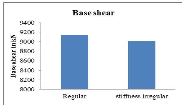
Chart -12: Base shear
