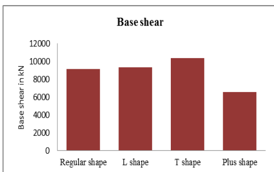
Chart -4: Base shear in X direction
