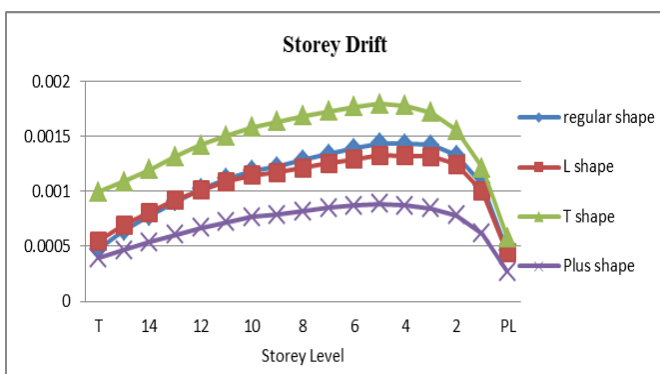
Chart -2: Storey drift in X direction
