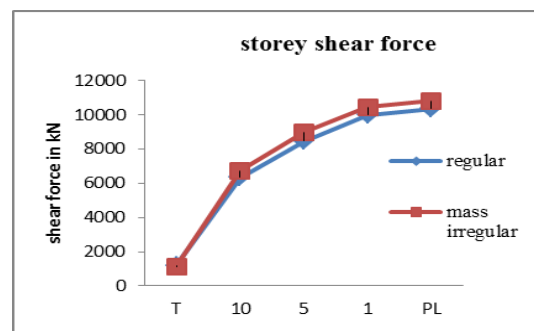
Chart -7: Storey shear force in X direction
