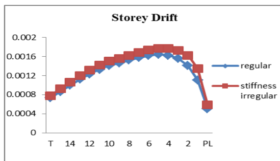
Chart -10: Storey drift in Y direction
