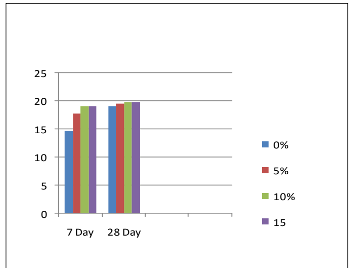
Fig. (b) Compressive Strength for M20 Grade Concrete
