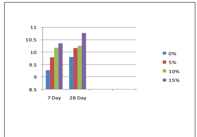
Fig. (e) Flexural Strength for M25 Grade Concrete
