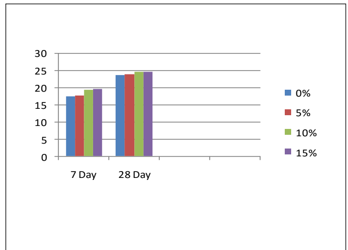
Fig. (c) Compressive Strength for M25 Grade Concrete
