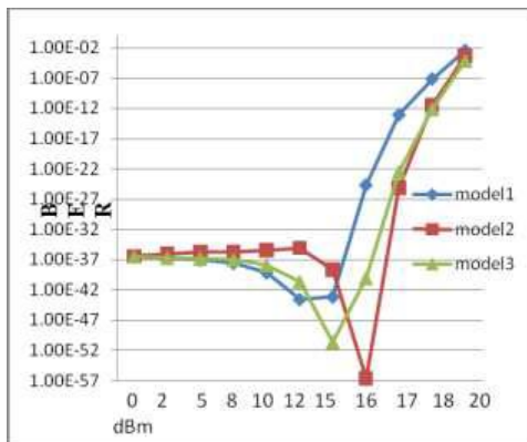
Figure 9: Comparison of transmission power vs. BER of three compensation system
