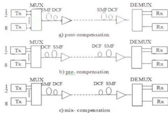
Figure 7: Three dispersion compensation techniques
