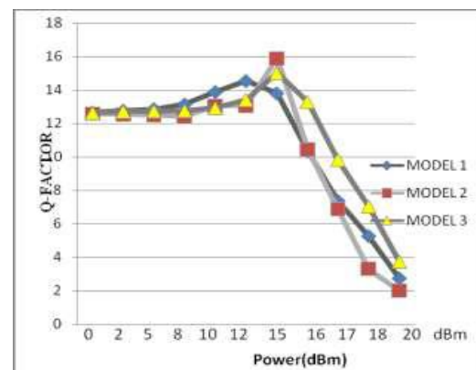
Figure 8: Comparison of transmission power vs. Q factor influence of three compensation system
