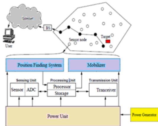
Fig 2. Sensor node
