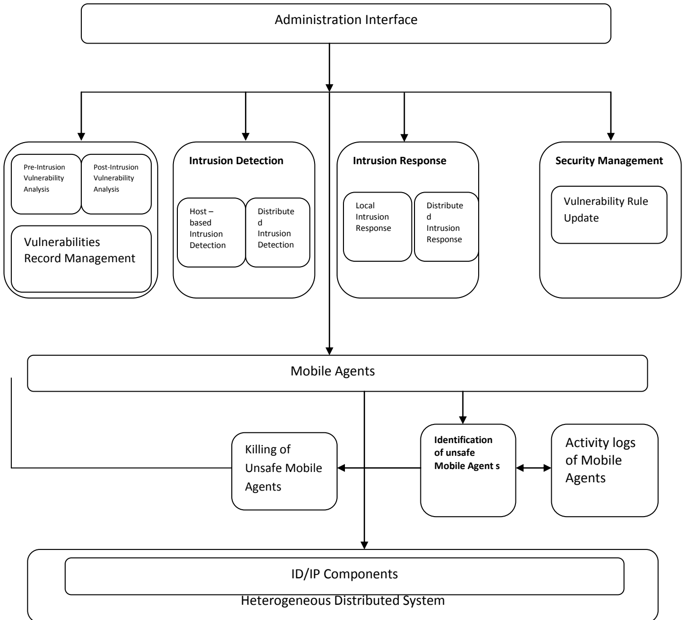
Fig -3: IDP System Layered Architecture
